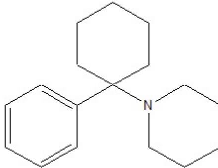
Phencyclidine
